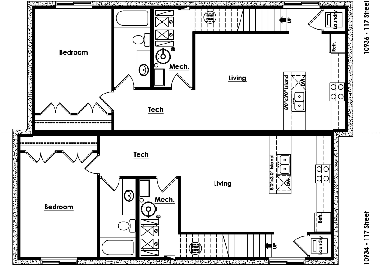
Foundation Plan/Basement Suite 651 sf
