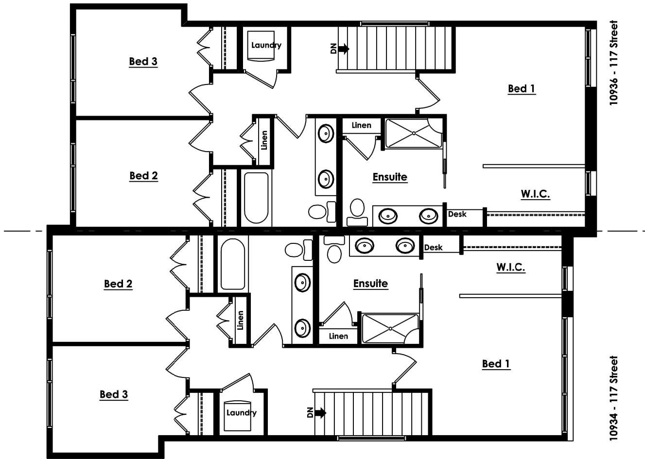
Second Floor Plan 781 sf
