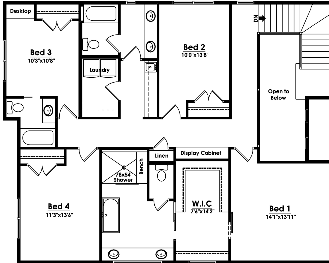
Second Floor Plan 1506 sf
